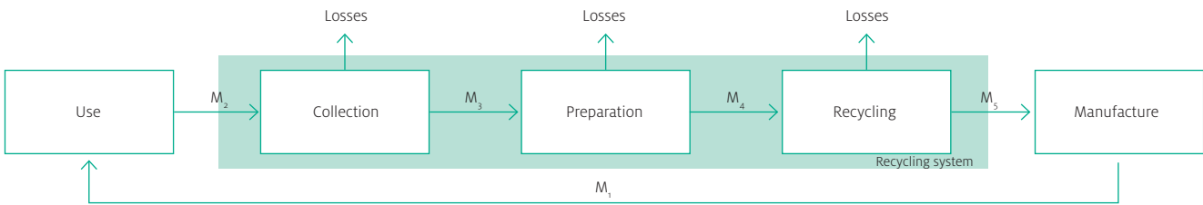
Figure 1: Simplified disposal system in which M_1 to M_5 represent total mass flows at a certain point in the processing chain. “Preparation” refers to all manual and mechanical processing procedures that generate final fractions for the last treatment stage, i.e. recycling.
